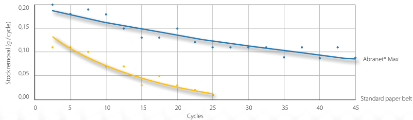
Abranet® Max vs Standard paper belt P120 – Oak sanding
